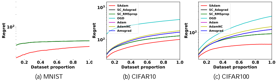
Fig. 1: Regret v.s. data proportion for \ell_2 -regularized softmax regression
